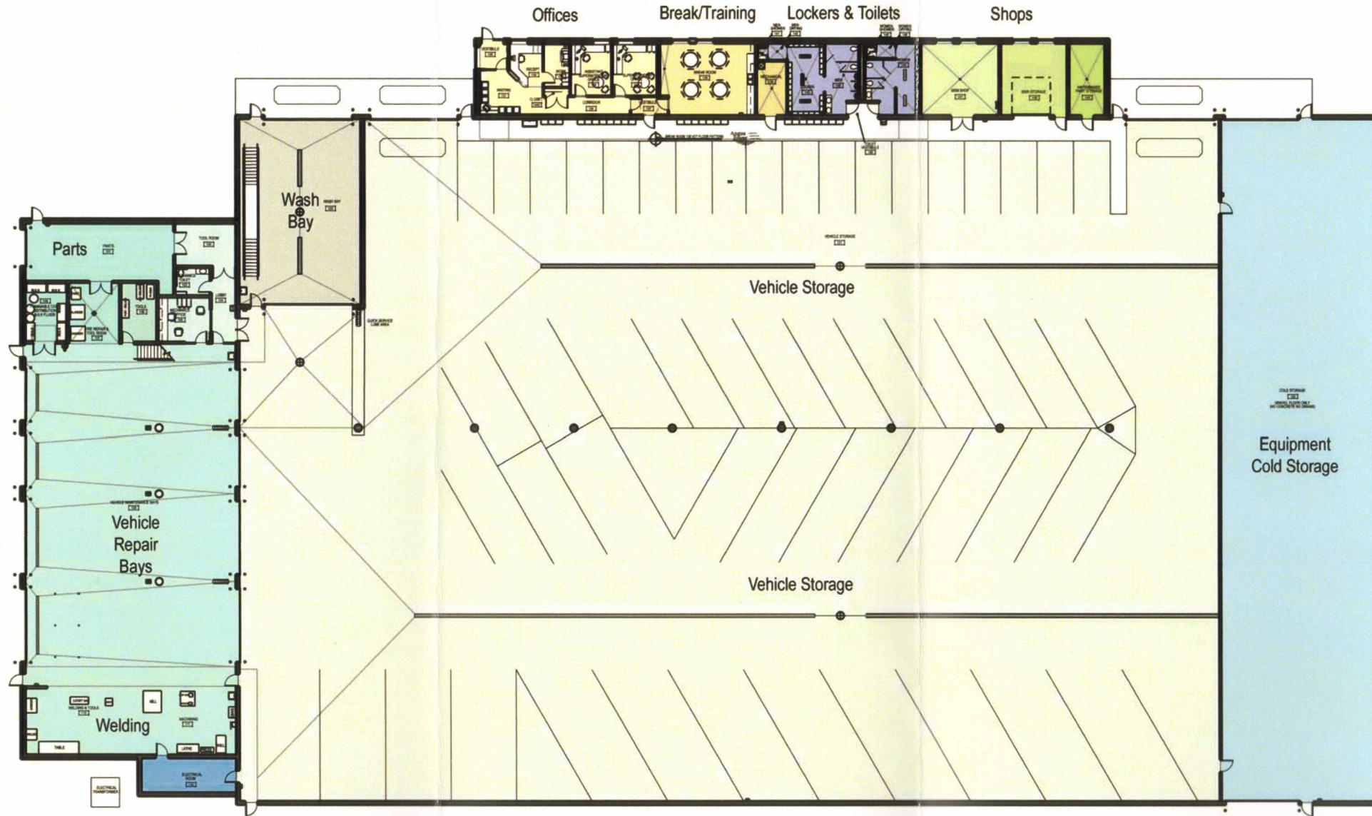
Floor Plan
